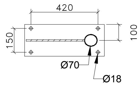
Base Plate
