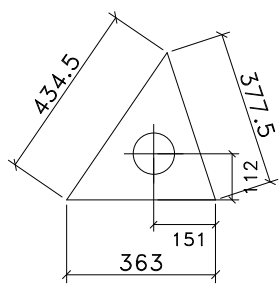
Stiffner
