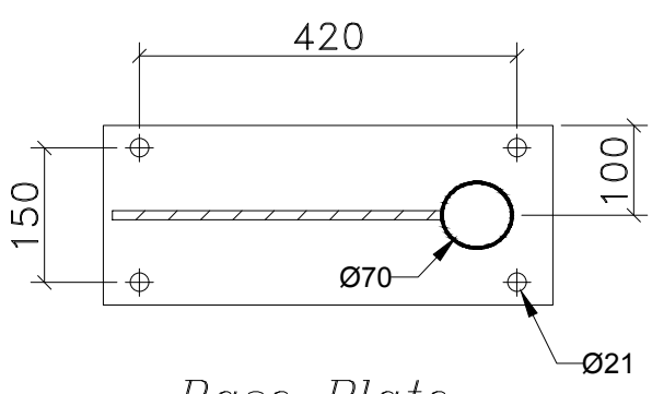
Base Plate
